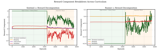
Fig. 7. Archived reward decomposition motivating reward-audit logging.
