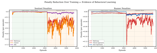
Fig. 6. Excluded legacy penalty traces; not comparable to the official v5 reward definition.
