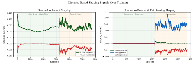
Fig. 7. Excluded legacy shaping traces; mechanism attribution requires the official tactical-reward ablation.
