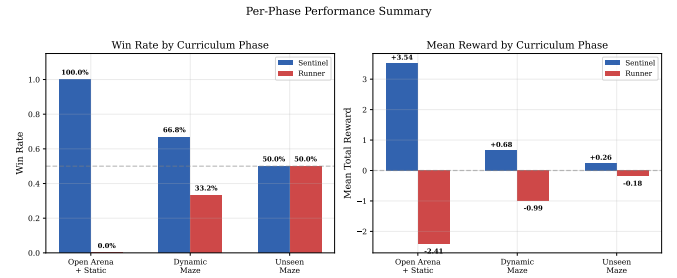
Fig. 8. Excluded legacy phase summary; it motivates but does not test the curriculum hypothesis.
