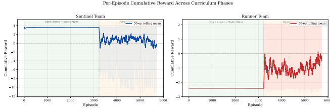
Fig. 3. Excluded legacy three-phase cumulative reward; not comparable to the official v5 curriculum.
