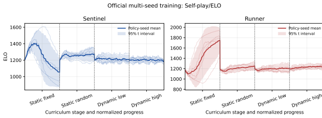
Fig. 2. Audited five-seed self-play ELO traces. Stable or increasing ELO does not imply Nash convergence; it is used as a training diagnostic.
