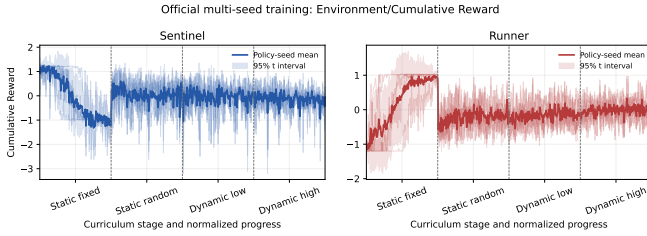
Fig. 1. Audited five-seed official curriculum reward curves exported from TensorBoard scalars. The official gate uses fixed trainer step budgets; the plotted curves are diagnostic summaries of completed training.
