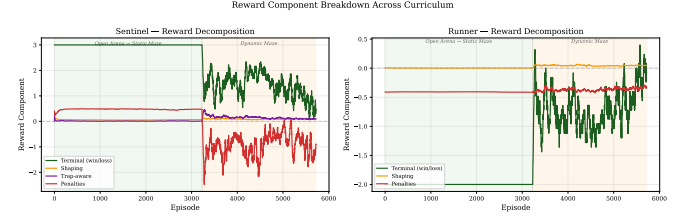
Fig. 4. Excluded legacy reward decomposition; not evidence about the official v5 weights.
