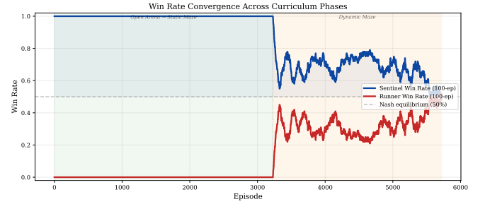
Fig. 5. Excluded legacy win-rate trace; descriptive history rather than an official comparison.
