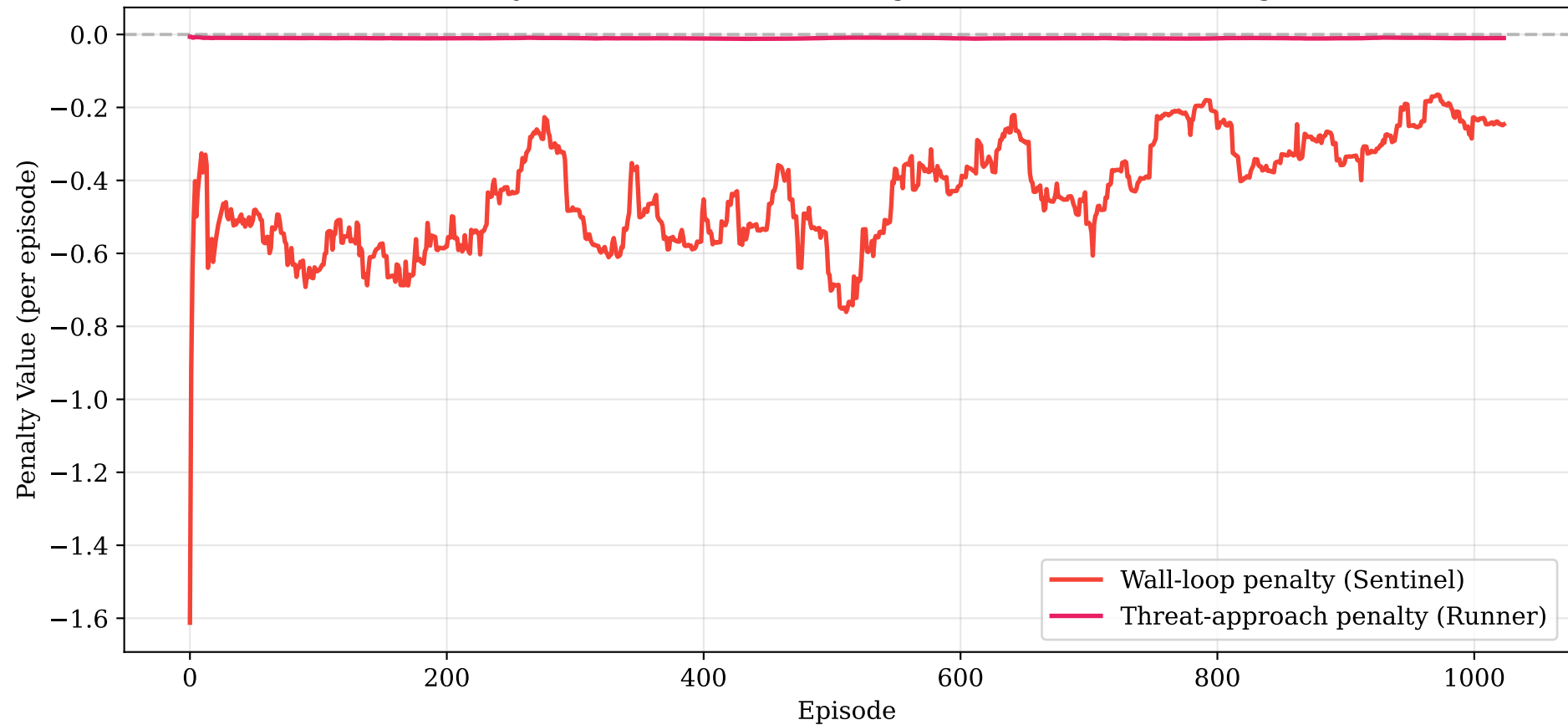
Penalty Reduction Over Training — Evidence of Learning
