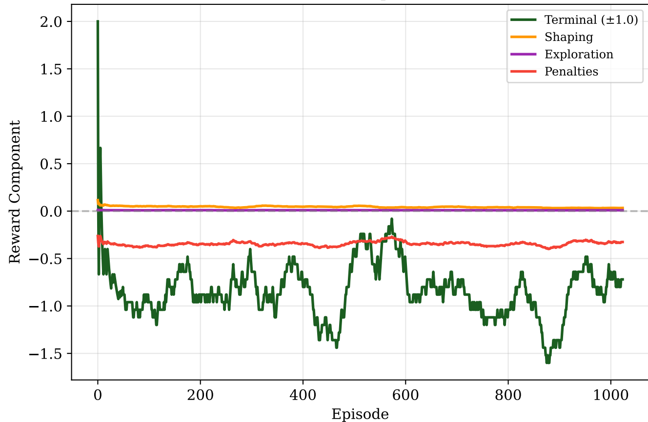
Runner — Reward Component Breakdown
