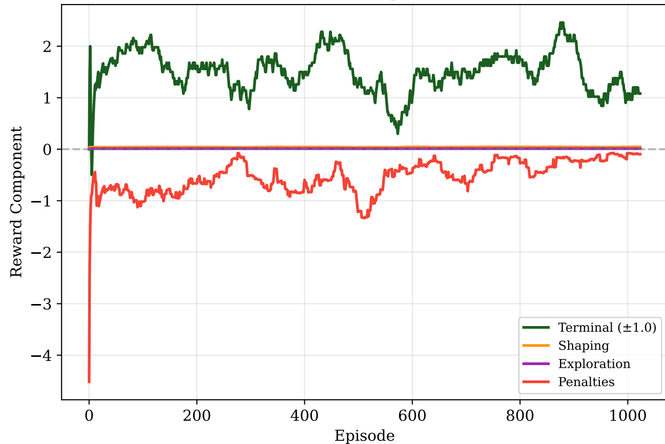
Sentinel — Reward Component Breakdown
