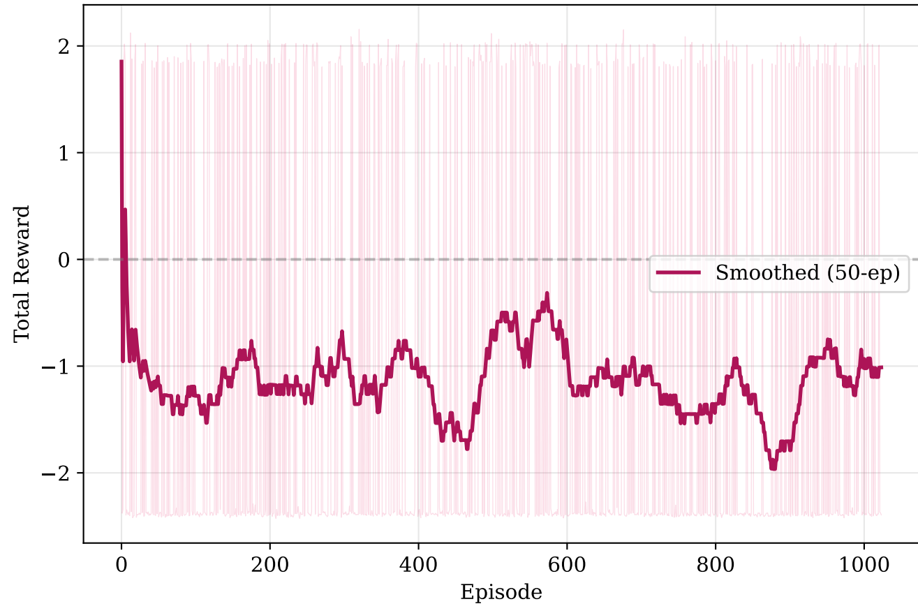
Runner Team — Cumulative Reward per Episode
