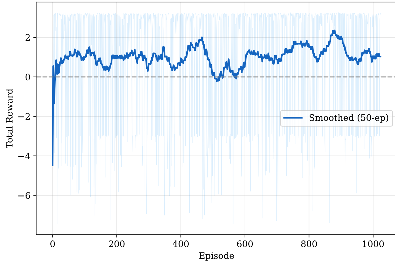
Sentinel Team — Cumulative Reward per Episode
