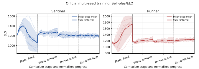
Fig. 3. Audited five-seed self-play ELO traces. Stable or increasing ELO does not imply Nash convergence; it is used as a training diagnostic.
