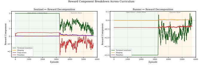
Fig. 5. Excluded legacy reward decomposition; not evidence about the official v5 weights.
