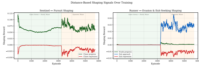
Fig. 8. Excluded legacy shaping traces; mechanism attribution requires the official tactical-reward ablation.
