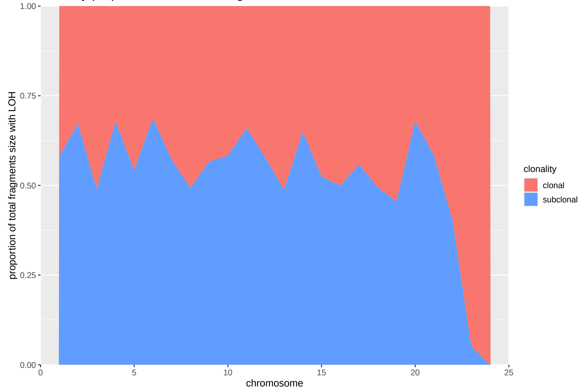
clonality proportion of the total fragment sizes with LOH in chromosomes
