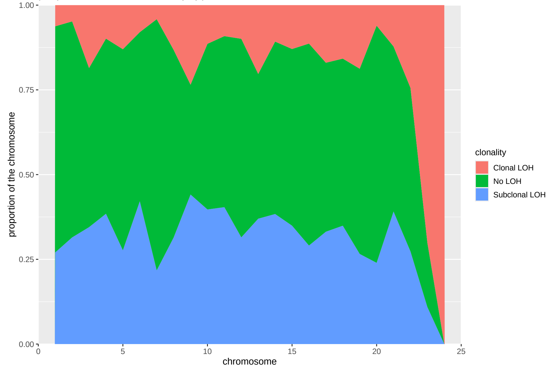
proportion of each clonality type in each chromosome in whole data studied
