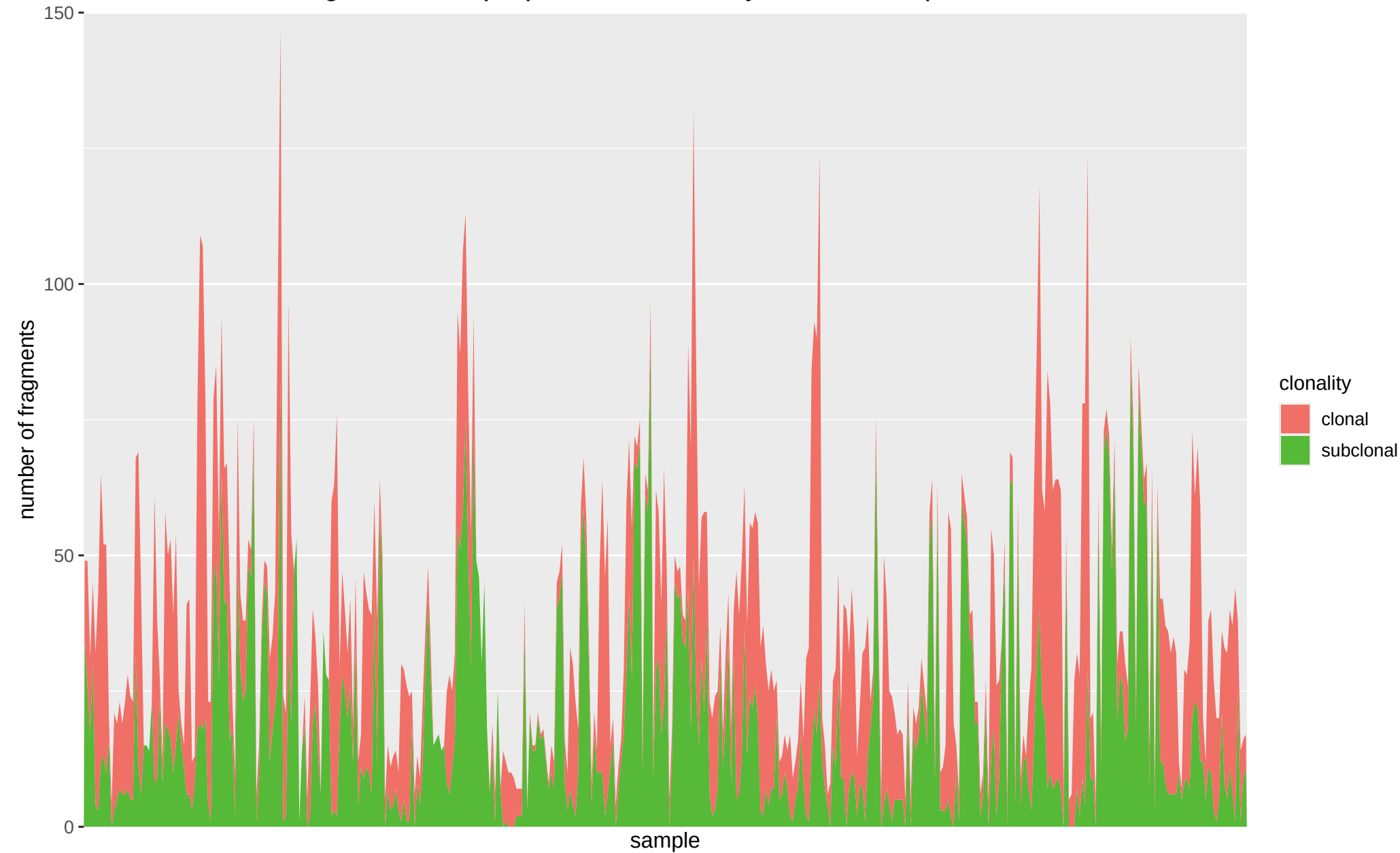
number of LOH fragments and proportion of clonality in each sample
