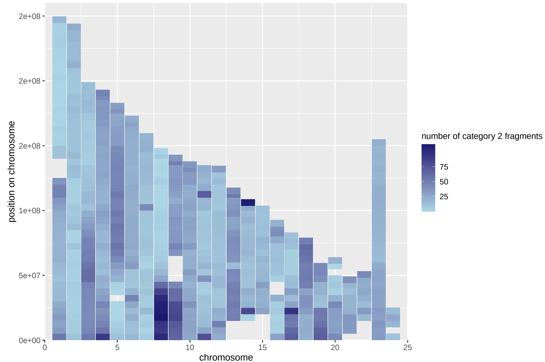
number of category 2 fragments in the genome of patients with LOH
