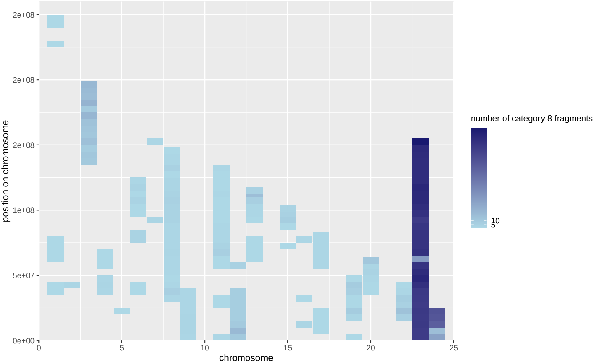
number of category 8 fragments in the genome of patients with LOH
