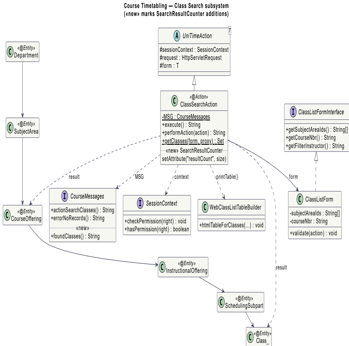
Figure 2 — Course Timetabling / Class Search class diagram
