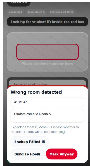
Wrong-room actions
