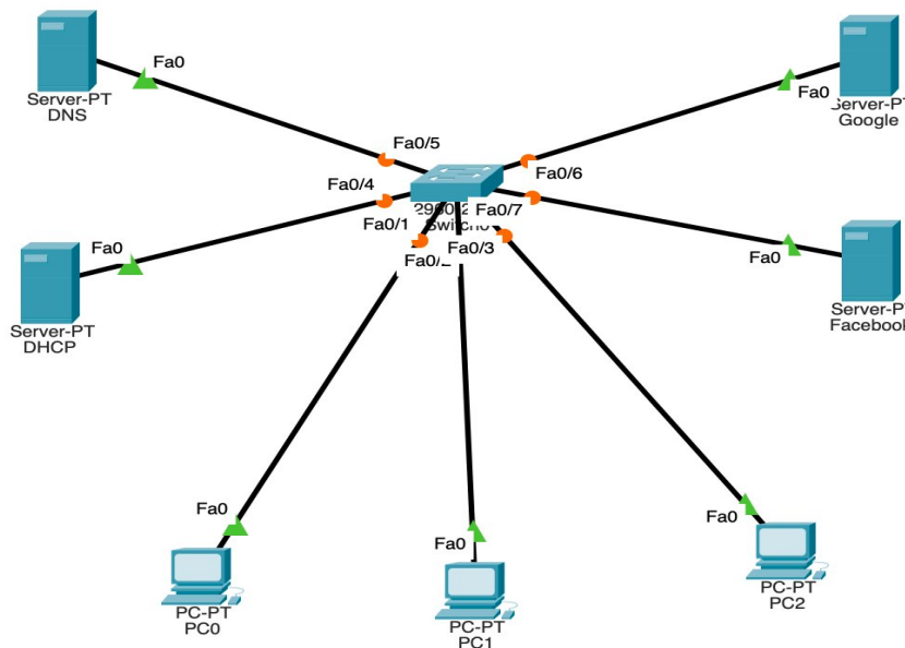
Figure 1 – Star topology: DNS, DHCP, Google, Facebook servers + PC0, PC1, PC2 on Switch0
