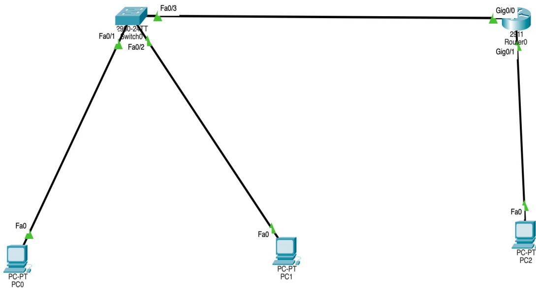
Figure 1 – Switch0 (PC0/PC1) → Router0 (2911) → PC2 direct on Gig0/1
