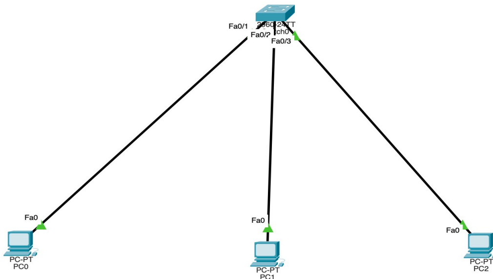
Figure 1 – Switch0 with PC0 (Fa0/1), PC1 (Fa0/2), PC2 (Fa0/3) on three VLANs
