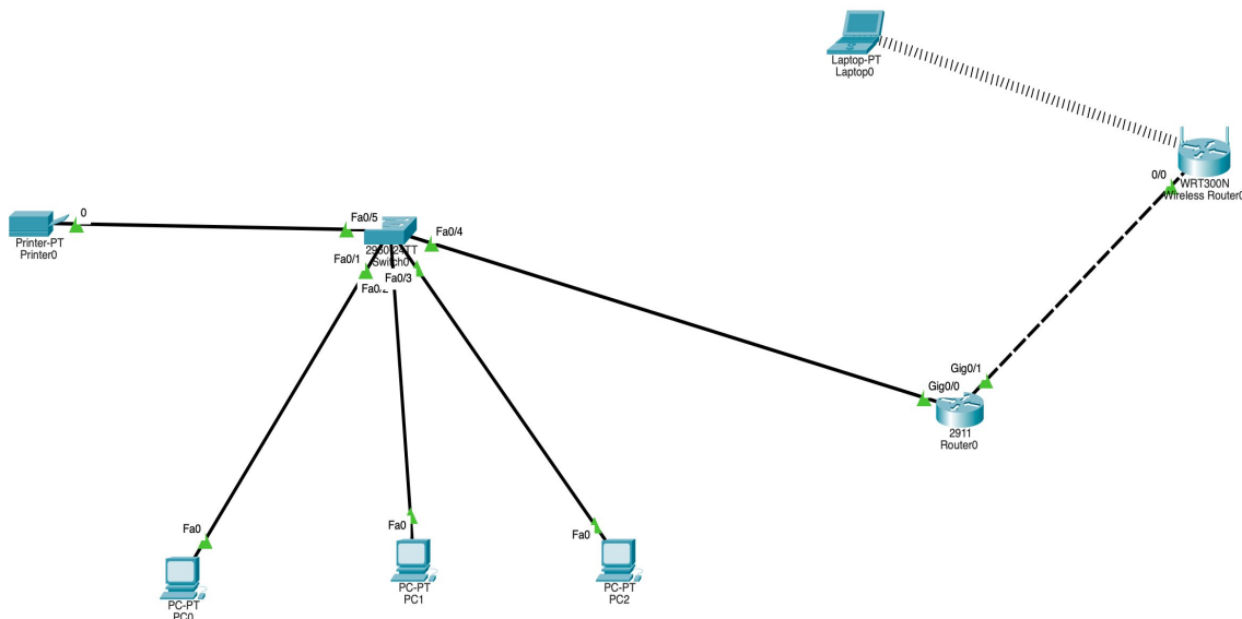
Figure 1 – Full topology: wired LAN (Switch0, PCs, Printer) + wireless (WRT300N, Laptop0)
