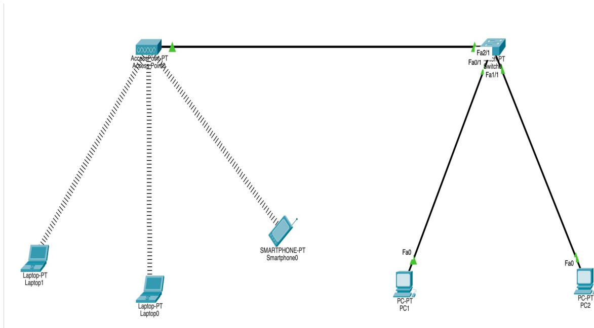
Figure 1 – Access Point, 3 wireless clients, Switch, PC1 & PC2
