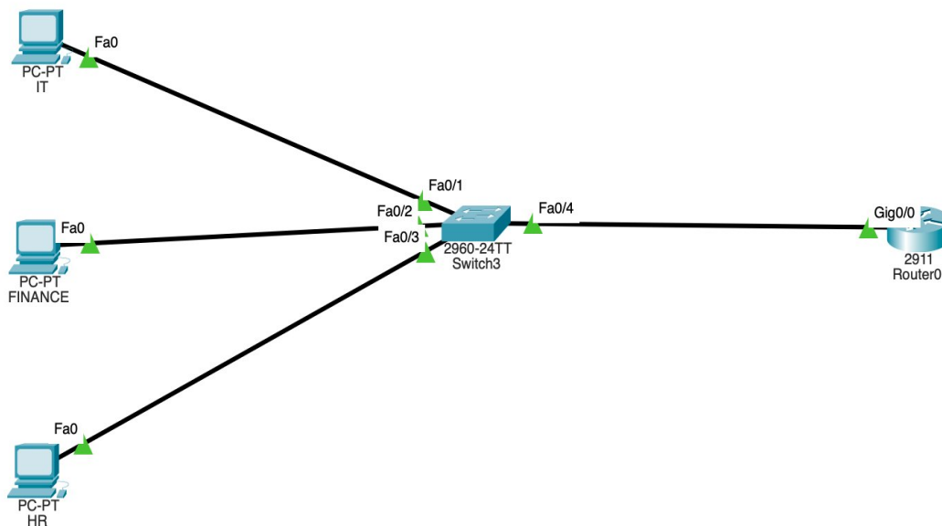
Figure 1 – IT, Finance, HR PCs on Switch3 connected to Router0 via trunk
