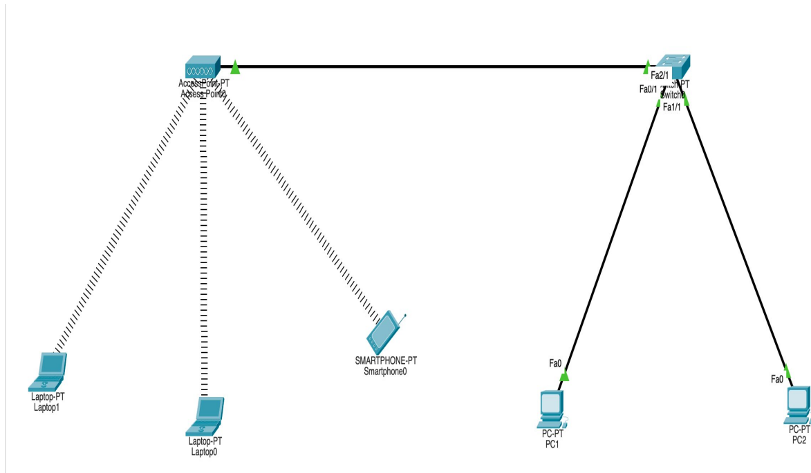
Figure 1 – Full topology: Access Point, wireless clients, Switch, PC1, PC2
