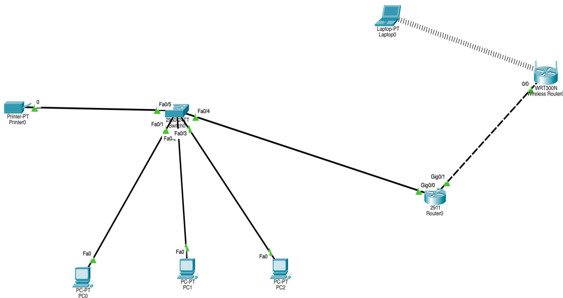
Figure 1 – Full topology: wired LAN (Switch0, PCs, Printer) + wireless (WRT300N, Laptop0)
