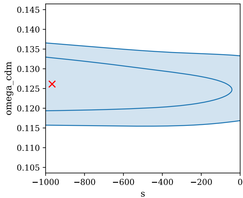
exotic DE on, datasets background
