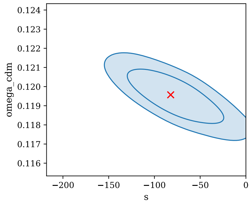
exotic DE on, datasets background + planck CMB
