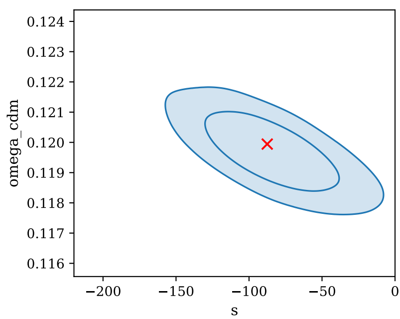
exotic DE on, datasets JWST CEERS + background + planck CMB fixed SHMR values, Full redshift range ( z \geq 9 )
