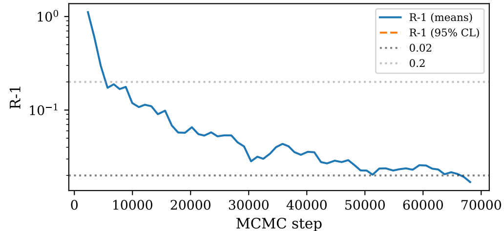
Convergence trajectory
