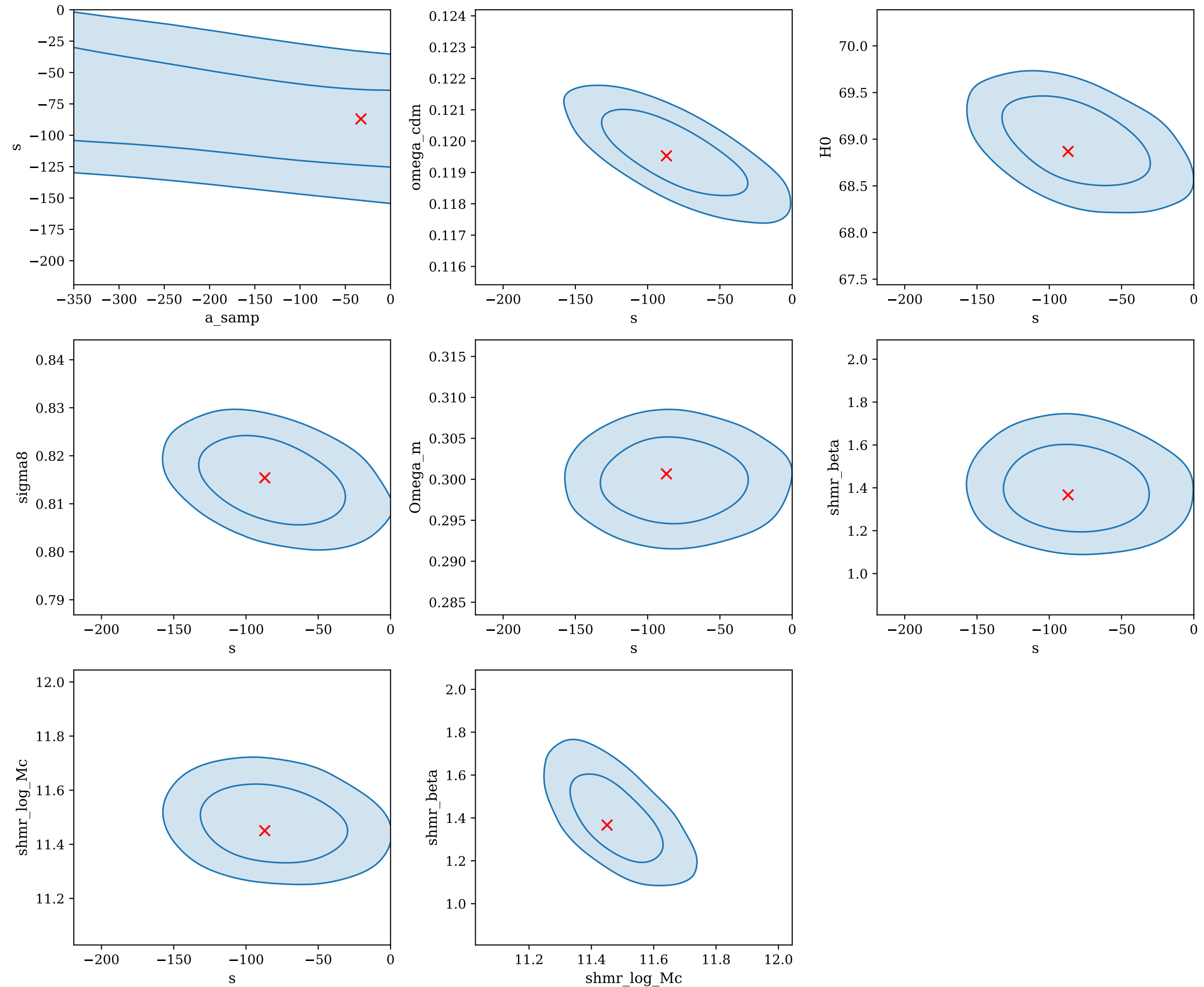
exotic DE on, datasets JWST CEERS + background + planck CMB varying SHMR, Full redshift range ( z \geq 9 )
