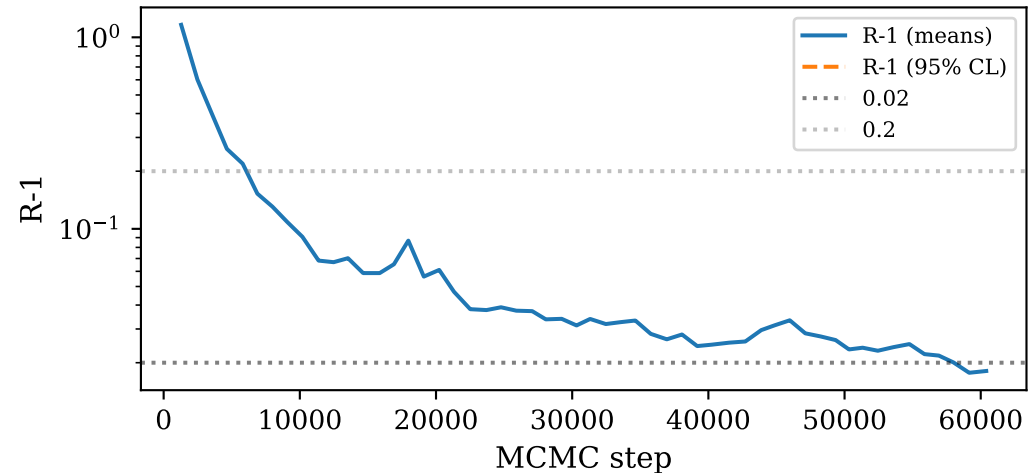
Convergence trajectory
