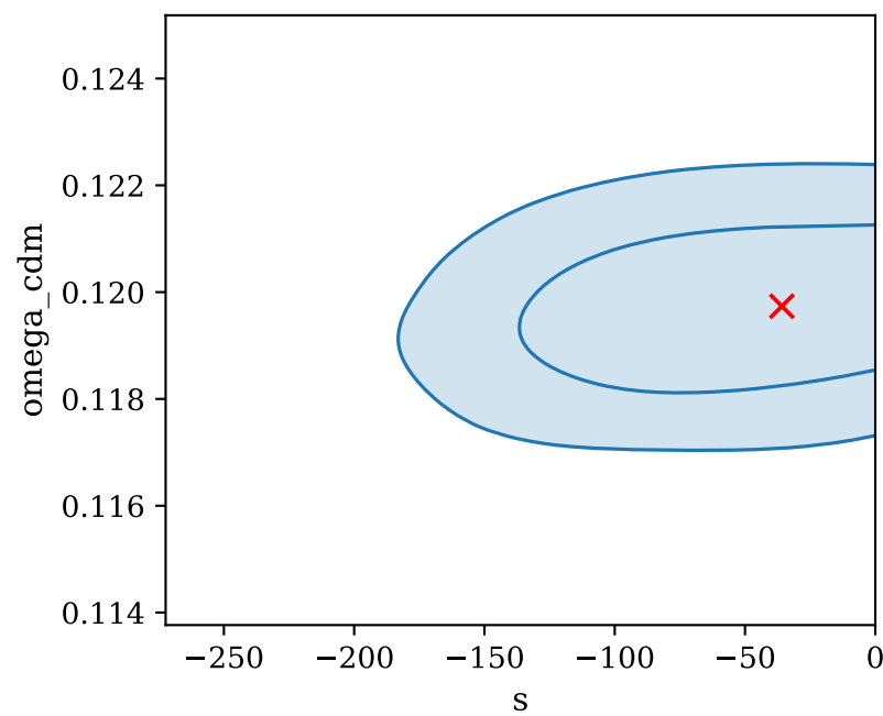
exotic DE on, datasets JWST PRIMER + planck CMB varying SHMR, Full redshift range ( z \geq 9 )
