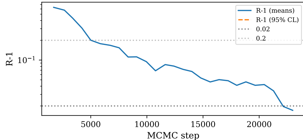
Convergence trajectory
