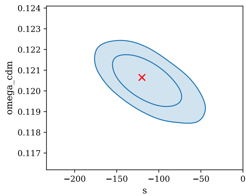
exotic DE on, datasets UVLF + background + planck CMB fixed SHMR values, Restricted redshift range ( z \geq 10 )
