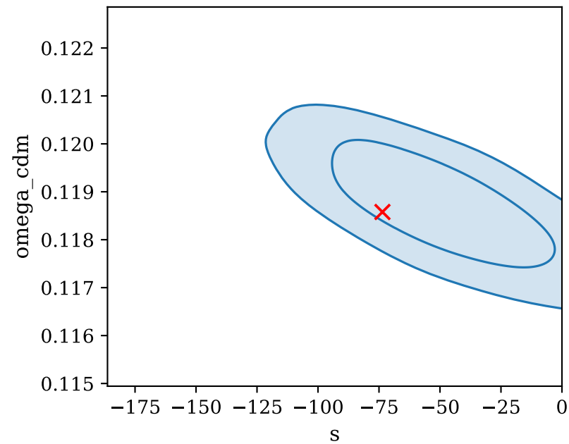
exotic DE on, datasets UVLF + background + planck CMB varying \beta , Full redshift range ( z \geq 9 )
