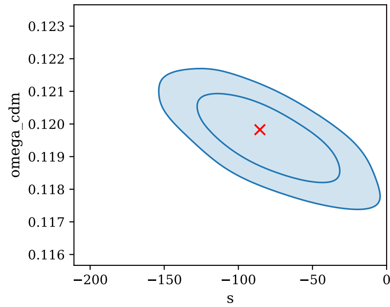
exotic DE on, datasets UVLF + background + planck CMB varying \beta , Restricted redshift range ( z \geq 10 )
