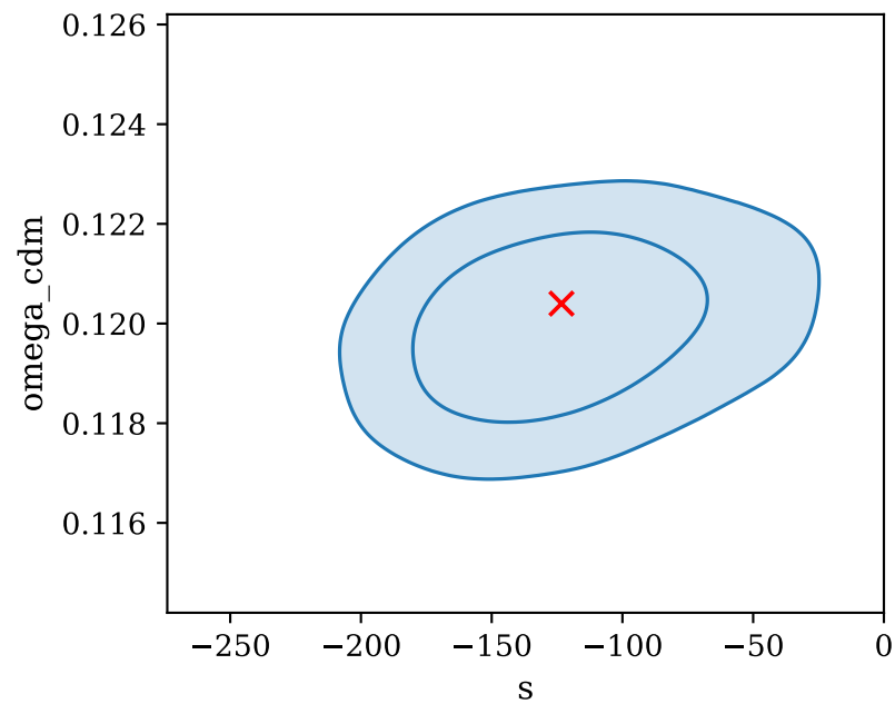
exotic DE on, datasets UVLF + planck CMB fixed SHMR values, Restricted redshift range ( z \geq 10 )
