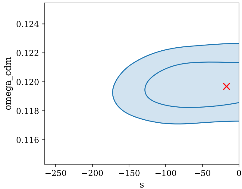
exotic DE on, datasets UVLF + planck CMB varying \beta , Restricted redshift range ( z \geq 10 )
