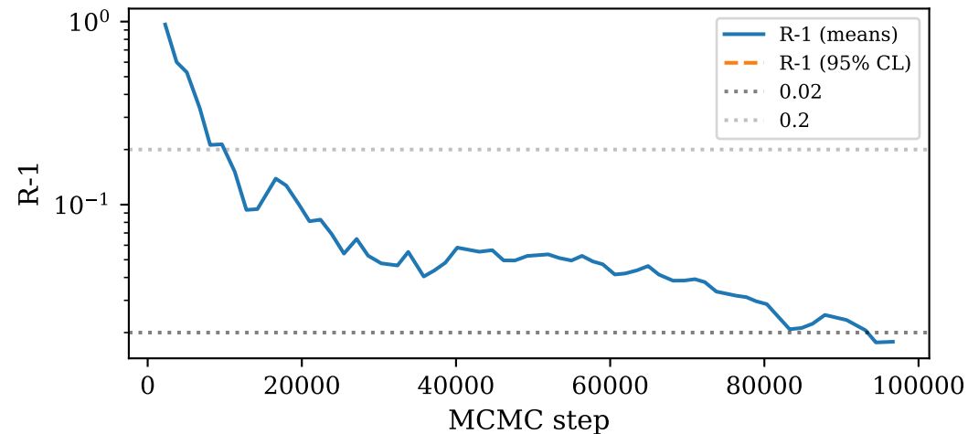
Convergence trajectory
