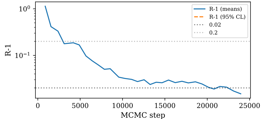
Convergence trajectory
