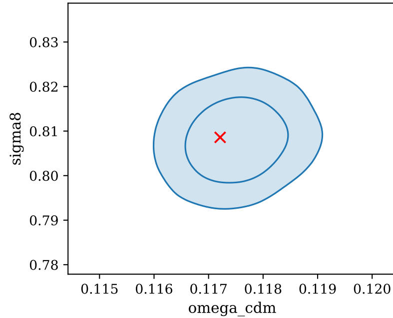
exotic DE off, datasets JWST CEERS + background + planck CMB varying SHMR, Full redshift range ( z \geq 9 )
