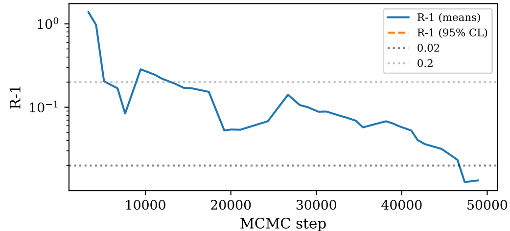
Convergence trajectory
