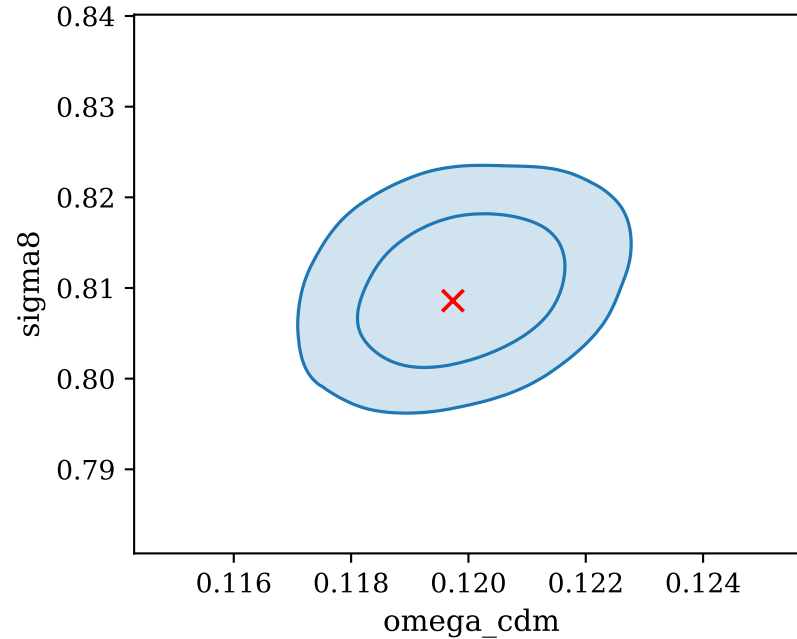
exotic DE off, datasets JWST PRIMER + planck CMB varying SHMR, Full redshift range ( z \geq 9 )
