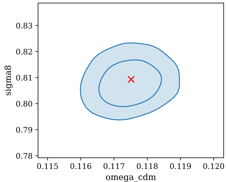
exotic DE off, datasets UVLF + background + planck CMB varying SHMR, Full redshift range ( z \geq 9 )
