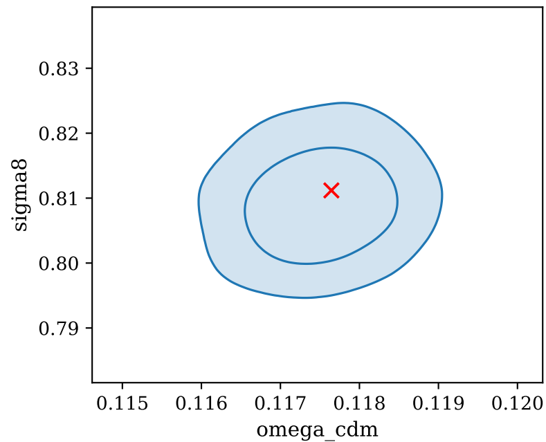
exotic DE off, datasets UVLF + background + planck CMB varying SHMR, Restricted redshift range ( z \geq 10 )
