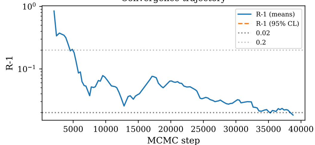
Convergence trajectory
