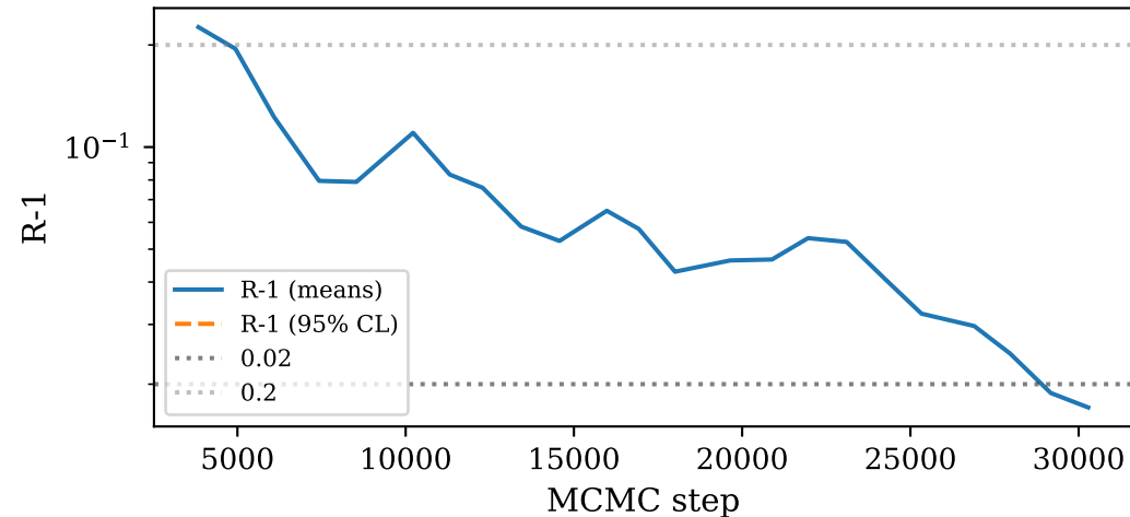
Convergence trajectory
