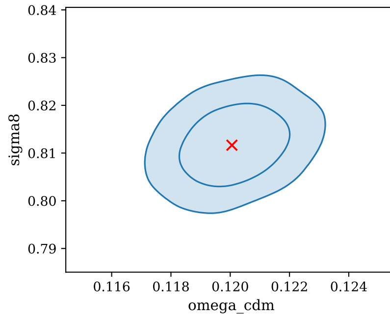
exotic DE off, datasets UVLF + planck CMB varying SHMR, Restricted redshift range ( z \geq 10 )
