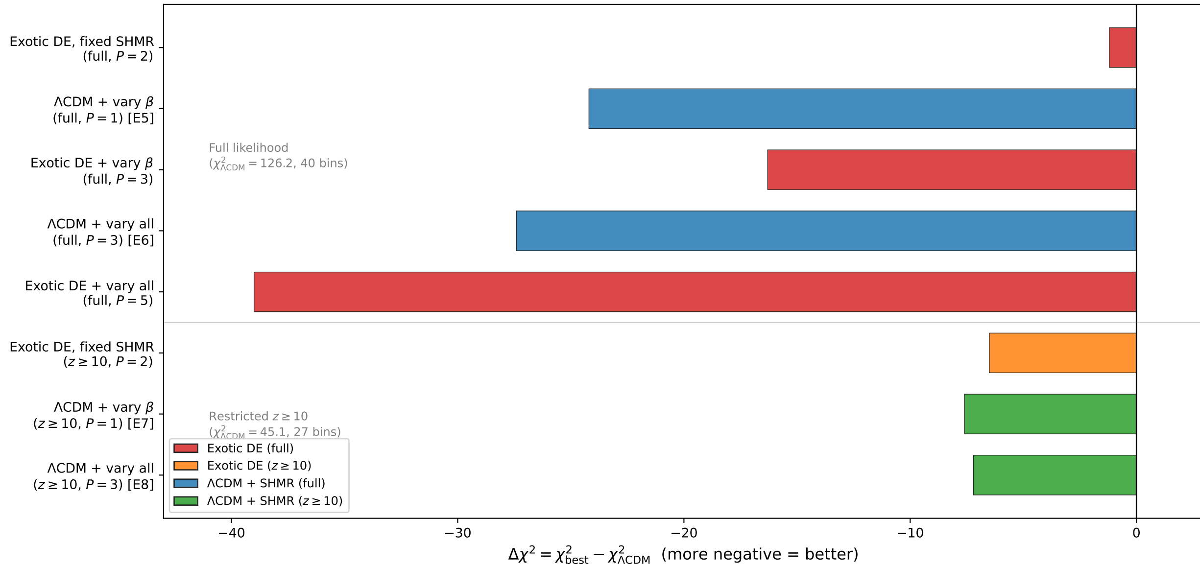
Minimisation results: Group B (GL + volume correction) + E5--E8 ( \Lambda CDM baselines)
