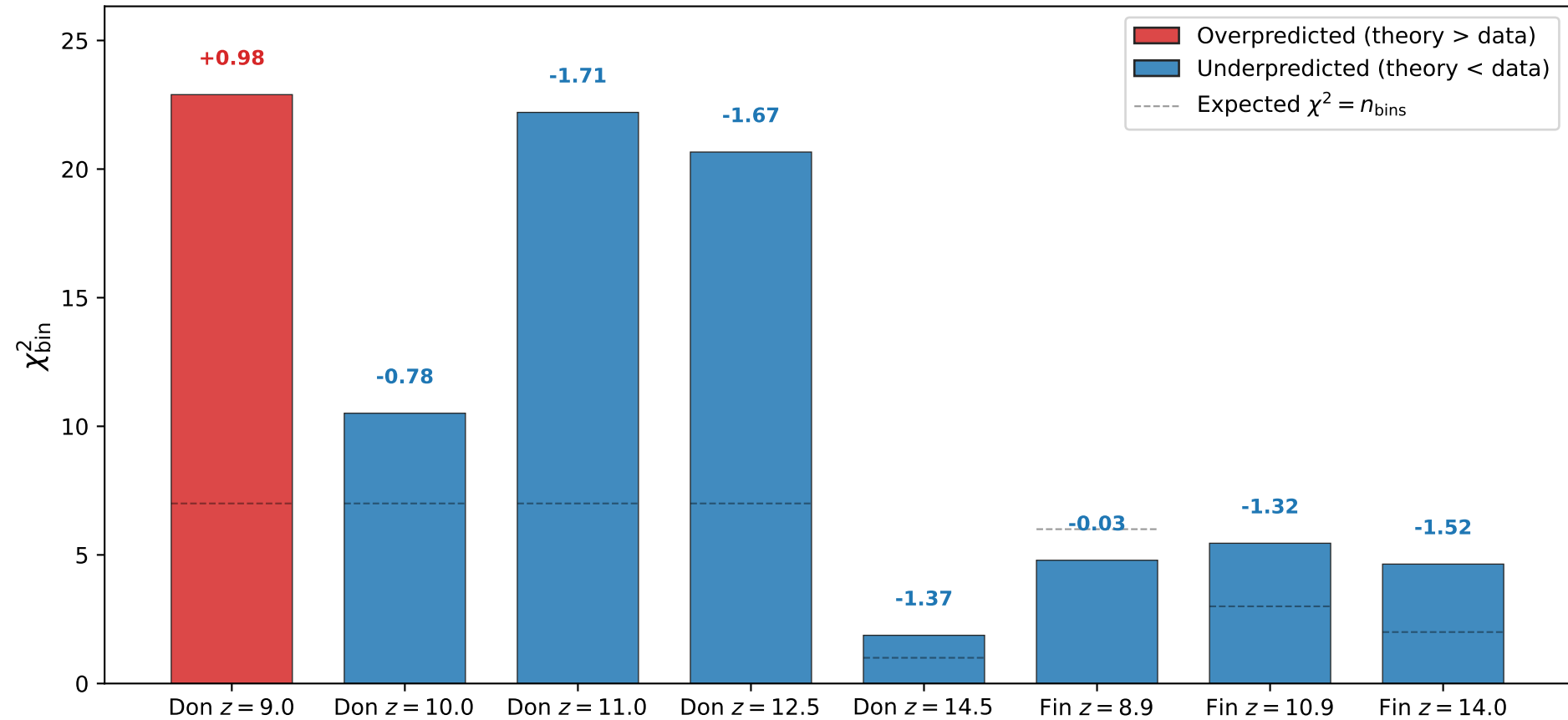
Per-bin \chi^2 at \Lambda CDM (with volume correction)
