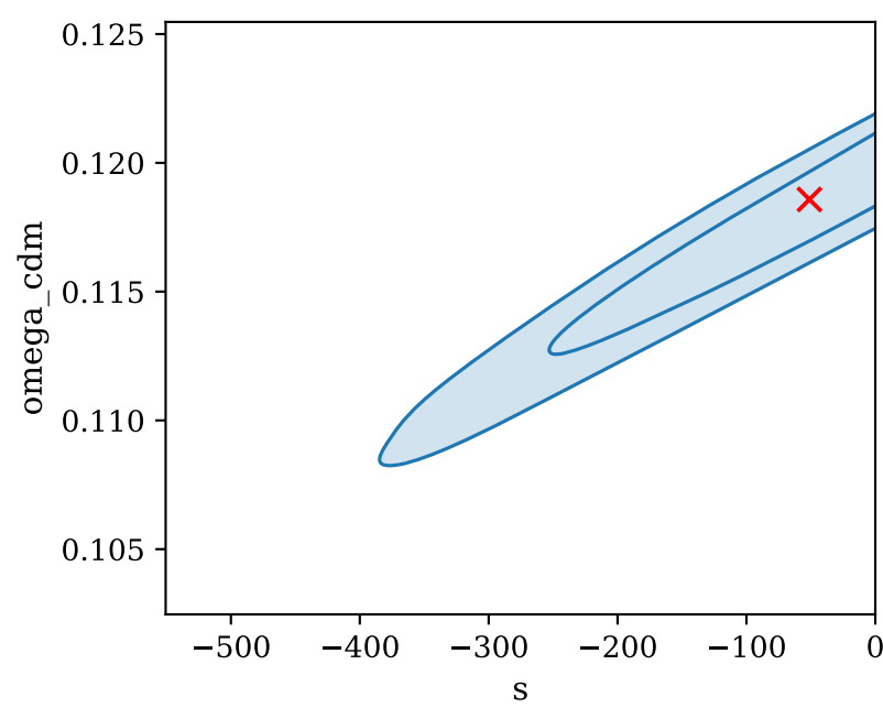
exotic DE on, datasets UVLF + background fixed SHMR values, Full redshift range ( z \geq 9 )
