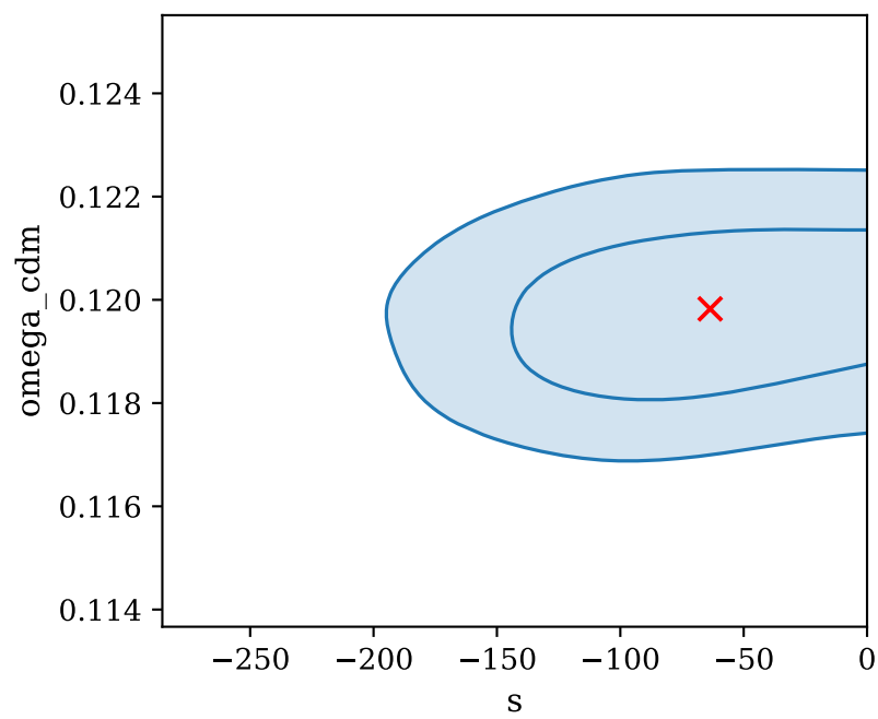
exotic DE on, datasets UVLF + planck CMB varying SHMR, Full redshift range ( z \geq 9 )
