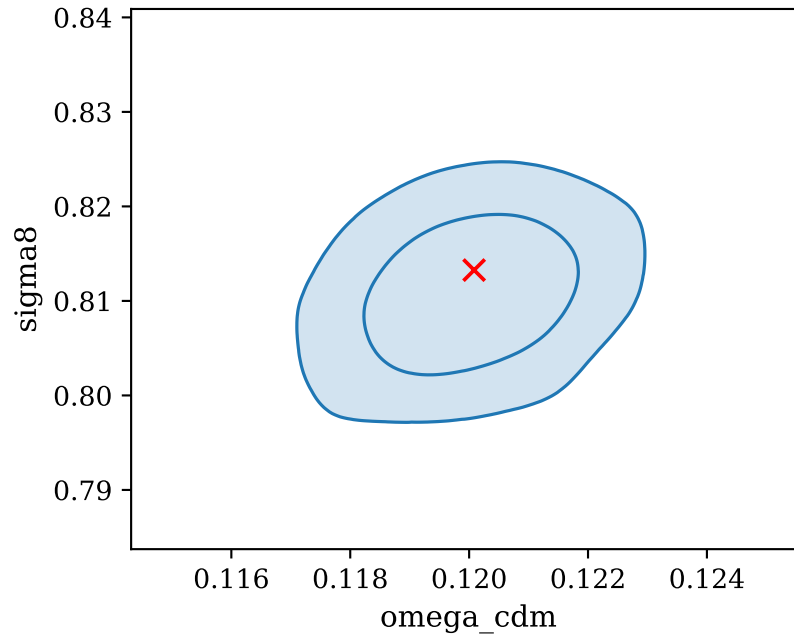
exotic DE off, datasets UVLF + planck CMB varying SHMR, Full redshift range ( z \geq 9 )
