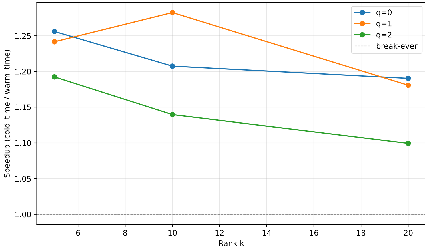
Timing Speedup vs Rank (p_warm=5)
